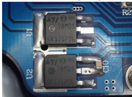
P2020160: L78 Voltage Regulator
